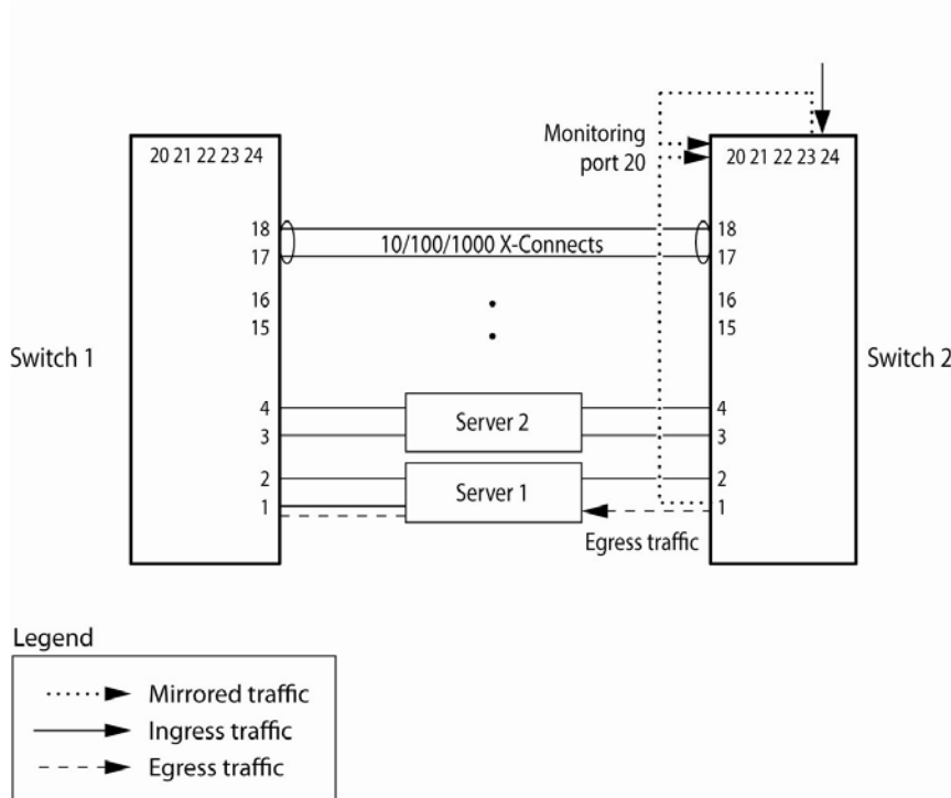
Figure 28 Port Mirroring
