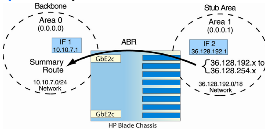
Figure 23 Summarizing routes
